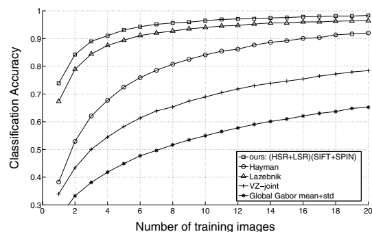
Figure 12. Comparison of different methods on the UIUCTex database.
